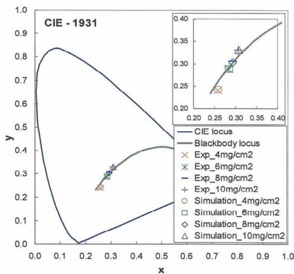
Figure 3 The simulated result verified the experimental result for the chromaticity coordinates in the blue light SPE package
