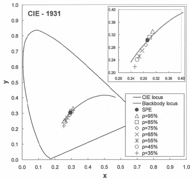
Figure 4 Chromaticity coordinates of the SPE package with transparent side surfaces compared with the remote phosphor package with reflective side surfaces with reflectances from 35% to 95%
