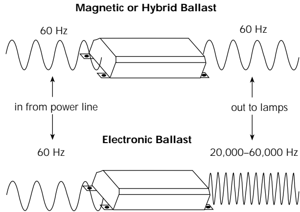
Figure 3. Operating Frequencies (in Hertz) of Ballasts
