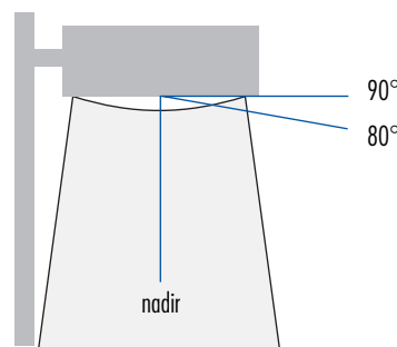
Figure 6. Angles Referenced by the IESNA Cutoff Classifications
